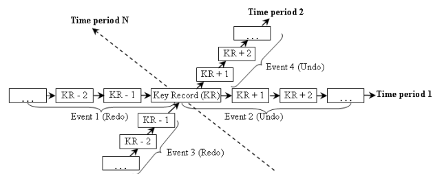
Figure 6: Result from Event Reconstruction (ER) process - autobiographic memory schema.
