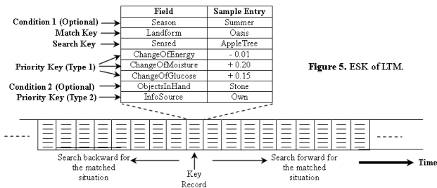
Figure 5: Event Specific Knowledge (ESK) of Long-term Memory (LTM).
