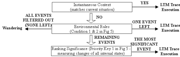
Figure 7: Event Filtering and Ranking (EFR) processes.
