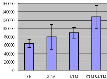
Figure 8: Experimental results with confidence values (error bars) showing the average lifespan of the 4 different agent control architectures running 10 times in each condition in the environment.
