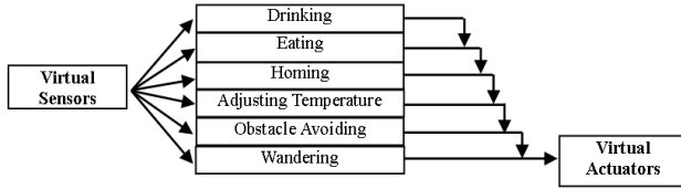
Figure 3: Behaviour hierarchy which is based on the subsumption architecture for a Purely Reactive (PR) agent.
