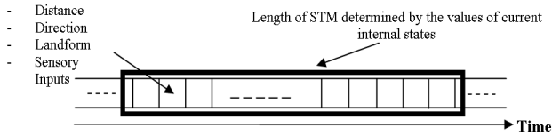
Figure 4: Short-term Memory (STM) with information indicating contents of each entry and the change of its length.
