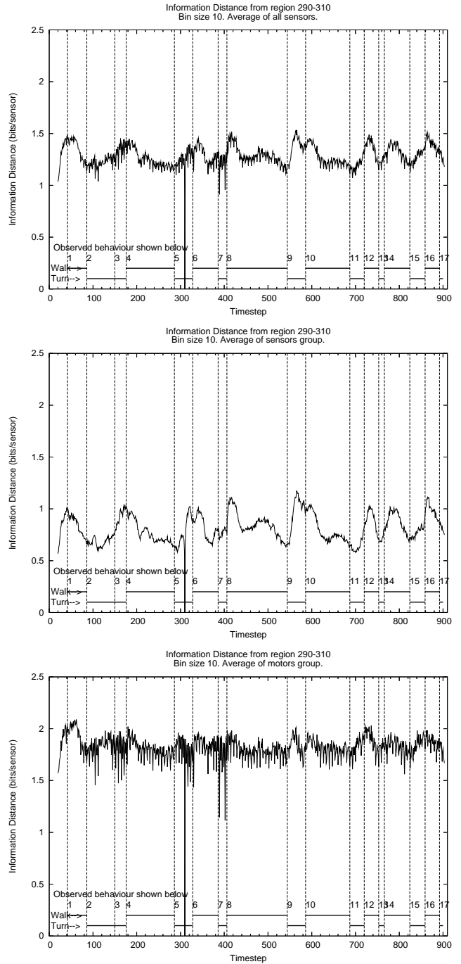
Figure 8: Information distances from region 290-310 (turning) to all other regions. Data from a robot exploring the environment. Time 290-310 corresponds to a part of a turn. For comparison, the observed behaviour is shown on the lower part of the graph with the vertical lines marking changes in behaviour. Top: All sensors, Middle: Exterioceptors, Bottom: Proprioceptors.
